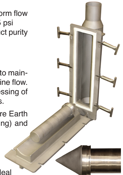
Stripper Collar
