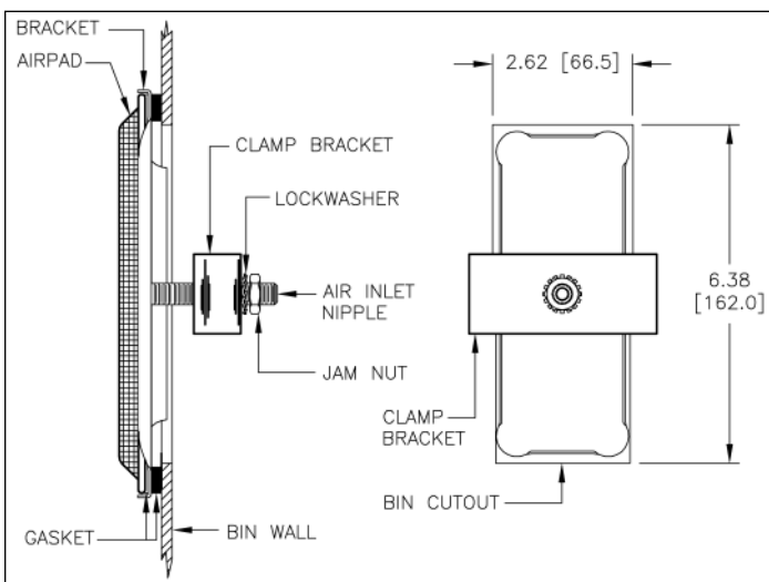
Use of External Mounting Kit
