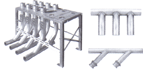
Manifolds & Stations
